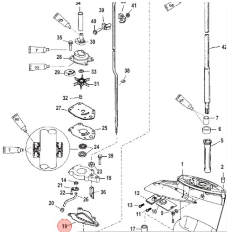
192043 - GASKET
