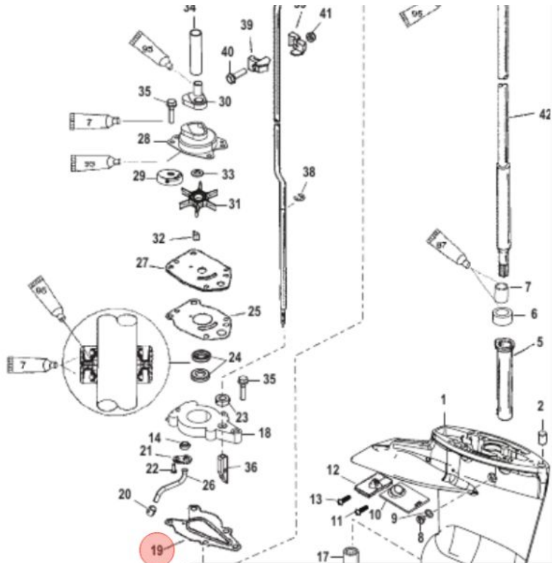
192043 - GASKET
